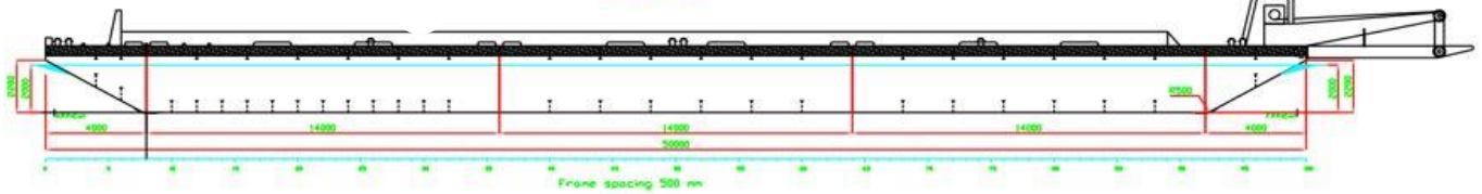
Side View
